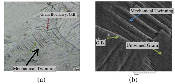
Fig. 4 a) Optical microscopy image; b) SEM image of tensile specimen of alloy 2 (near the fractured surface)
